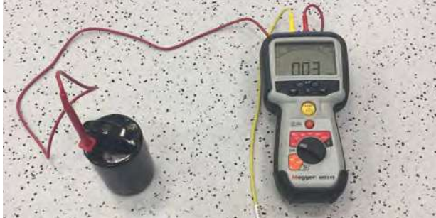
Figure 7.3 Test electrode
