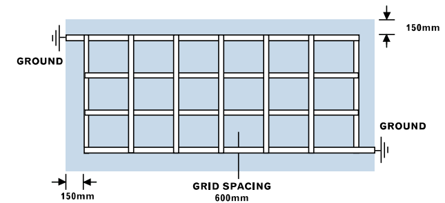
Figure 7.2 Earth strip layout
