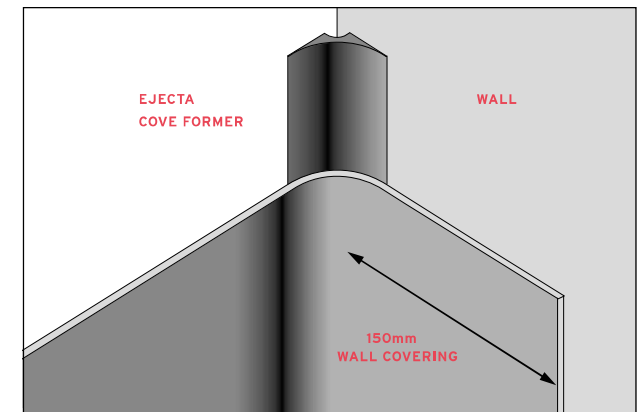
Figure 8.1 Ejecta cover former
