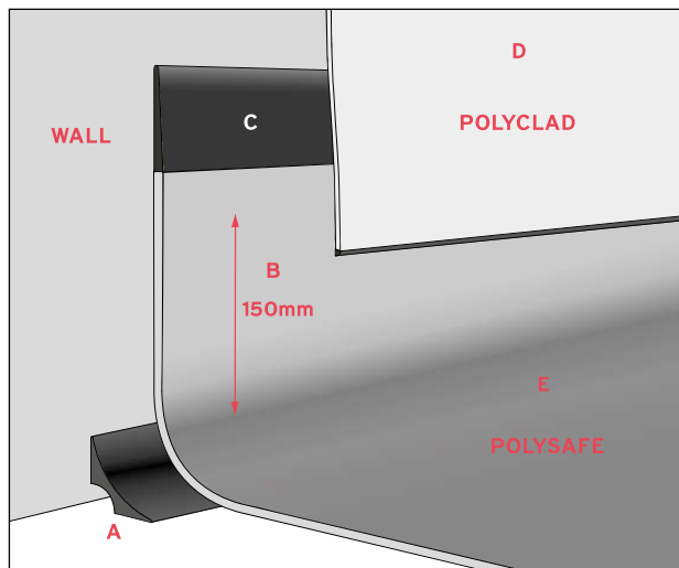
Figure 8.2 Overlap installation method
